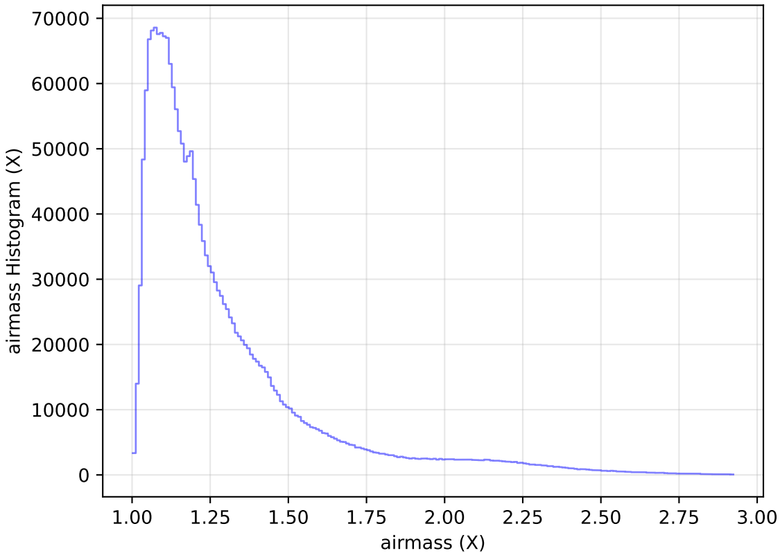
smc_lmc_v3.3_10yrs All sky all bands: airmass Histogram
