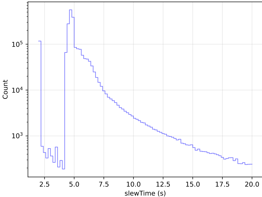
smc_lmc_v3.3_10yrs All visits: Zoom Slew Time Histogram
