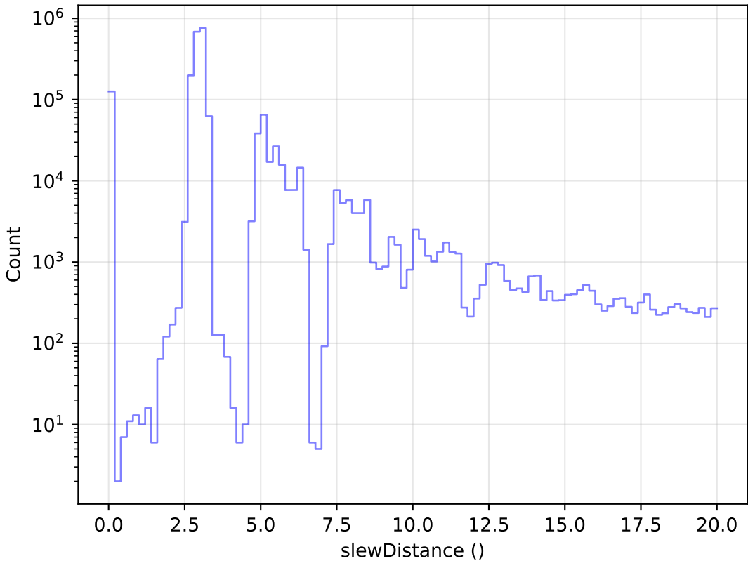
smc_lmc_v3.3_10yrs All visits: Zoom Slew Distance Histogram
