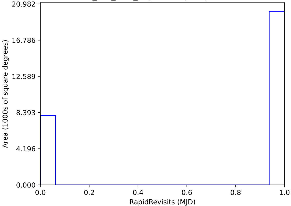
smc_lmc_v3.3_10yrs All sky: RapidRevisits
