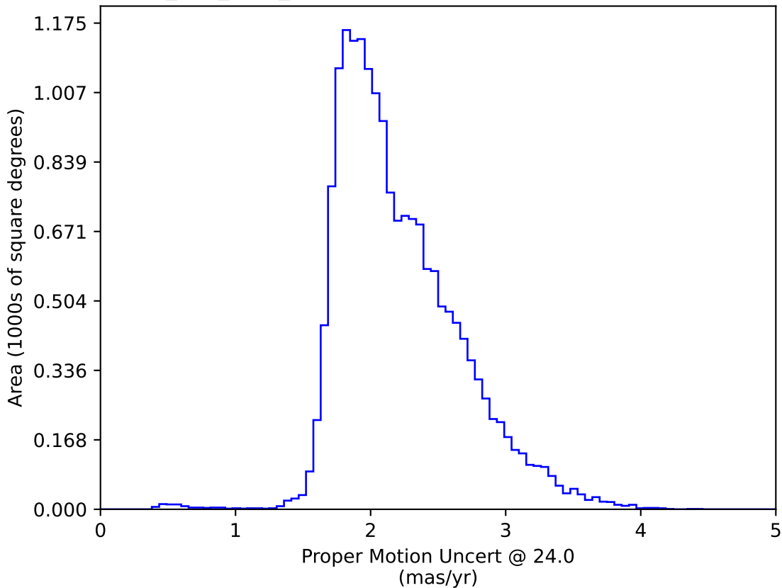
smc_lmc_v3.3_10yrs WFD: Proper Motion Uncert @ 24.0
