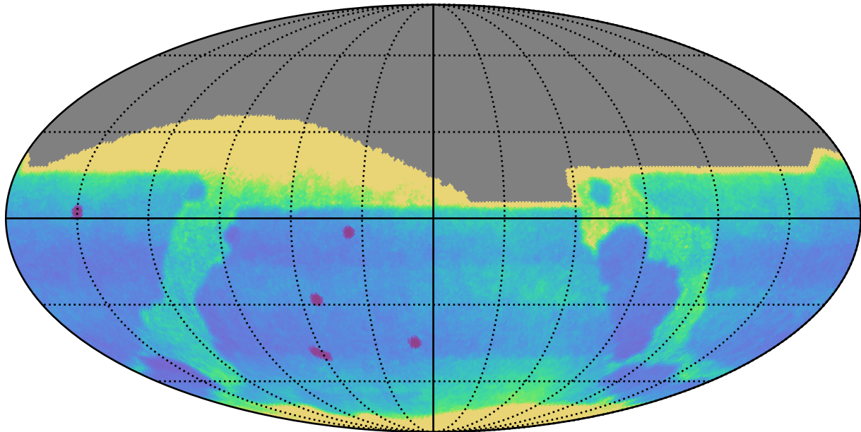
smc_lmc_v3.3_10yrs All sky: Proper Motion Uncert @ 24.0
