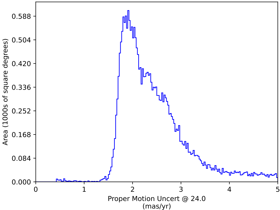
smc_lmc_v3.3_10yrs All sky: Proper Motion Uncert @ 24.0
