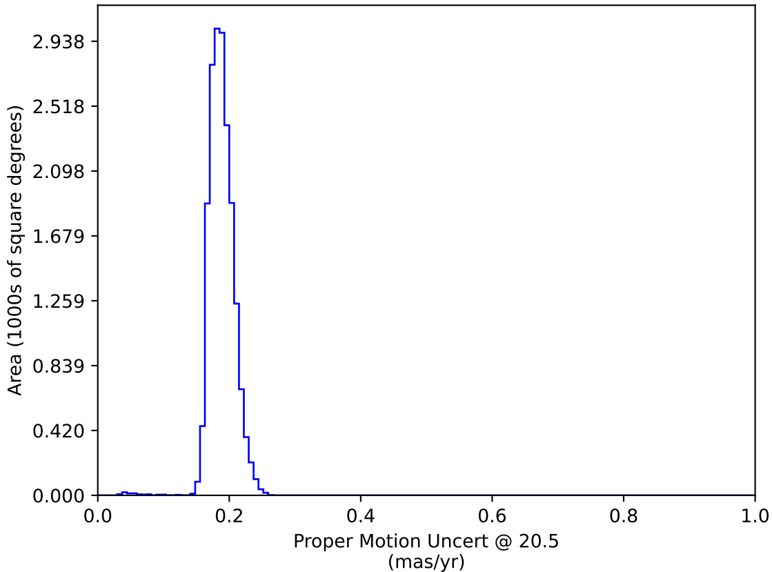
smc_lmc_v3.3_10yrs WFD: Proper Motion Uncert @ 20.5
