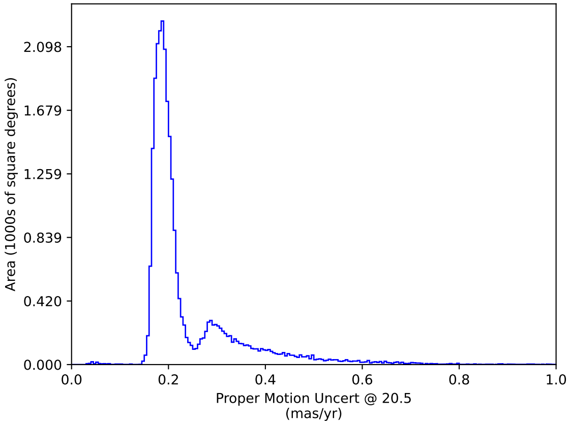
smc_lmc_v3.3_10yrs All sky: Proper Motion Uncert @ 20.5
