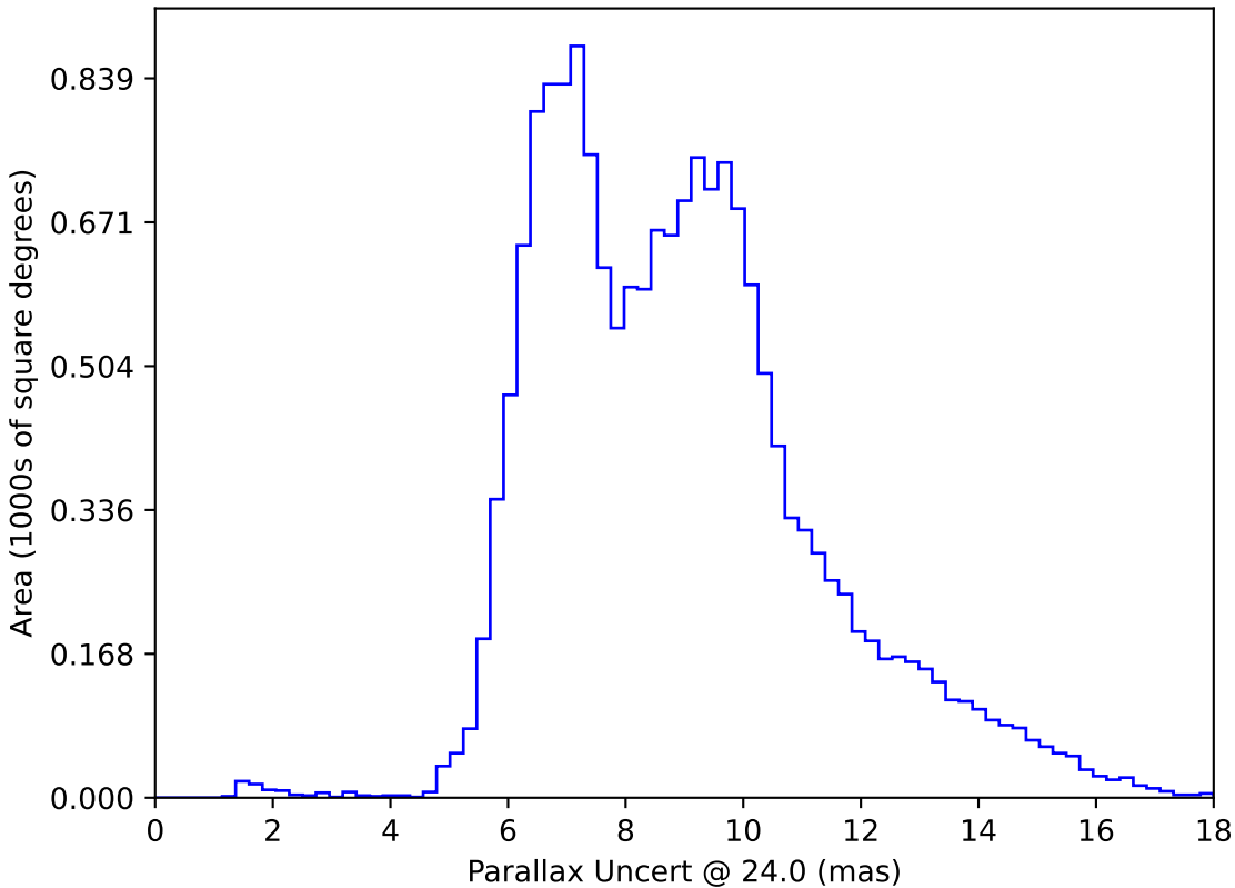
smc_lmc_v3.3_10yrs WFD: Parallax Uncert @ 24.0
