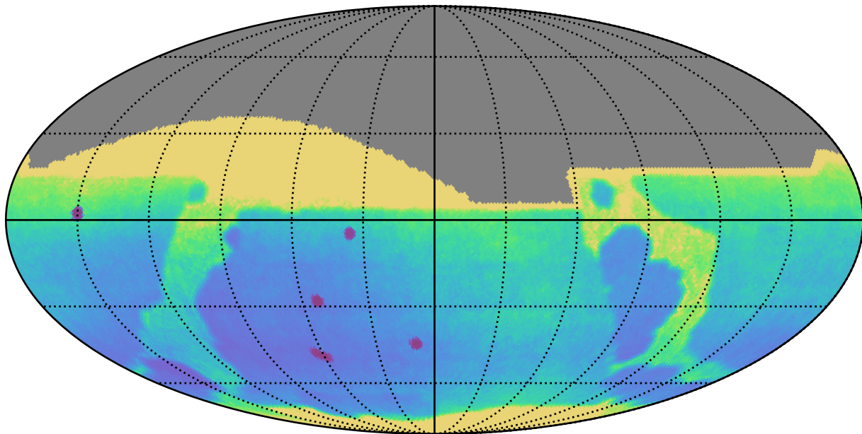
smc_lmc_v3.3_10yrs All sky: Parallax Uncert @ 24.0
