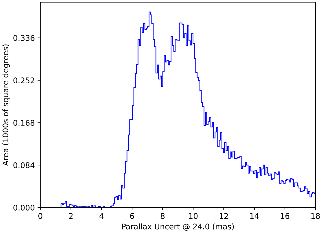
smc_lmc_v3.3_10yrs All sky: Parallax Uncert @ 24.0
