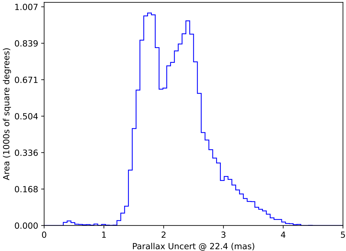
smc_lmc_v3.3_10yrs WFD: Parallax Uncert @ 22.4
