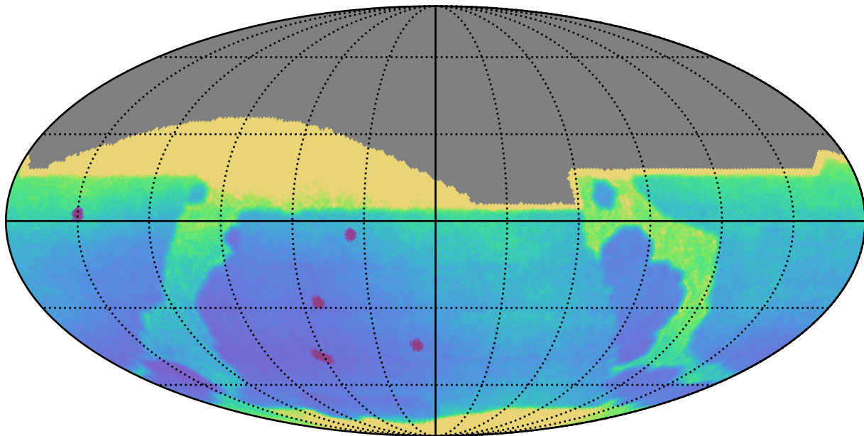
smc_lmc_v3.3_10yrs All sky: Parallax Uncert @ 22.4
