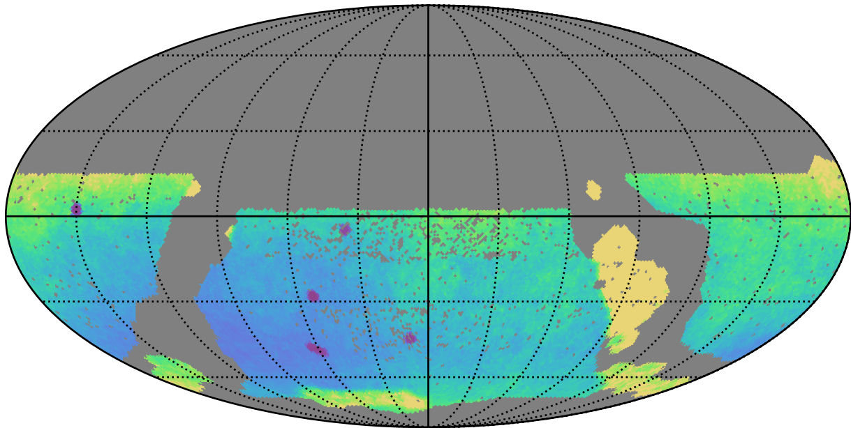
smc_lmc_v3.3_10yrs WFD y band only: Parallax Uncert @ 21.3
