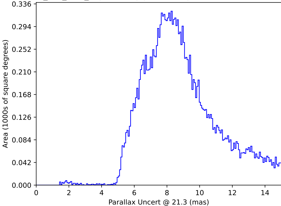
smc_lmc_v3.3_10yrs All sky y band only: Parallax Uncert @ 21.3
