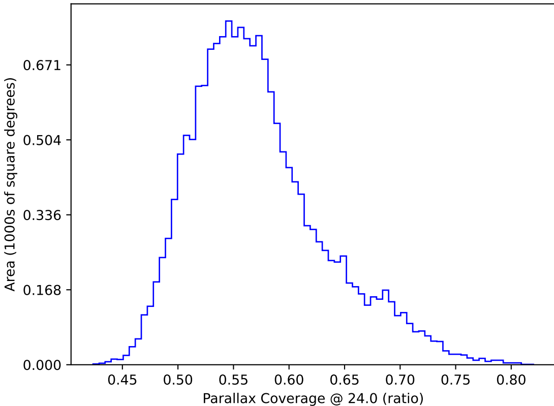
smc_lmc_v3.3_10yrs WFD: Parallax Coverage @ 24.0
