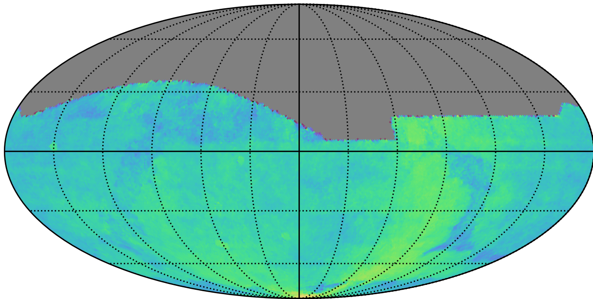
smc_lmc_v3.3_10yrs All sky: Parallax Coverage @ 24.0
