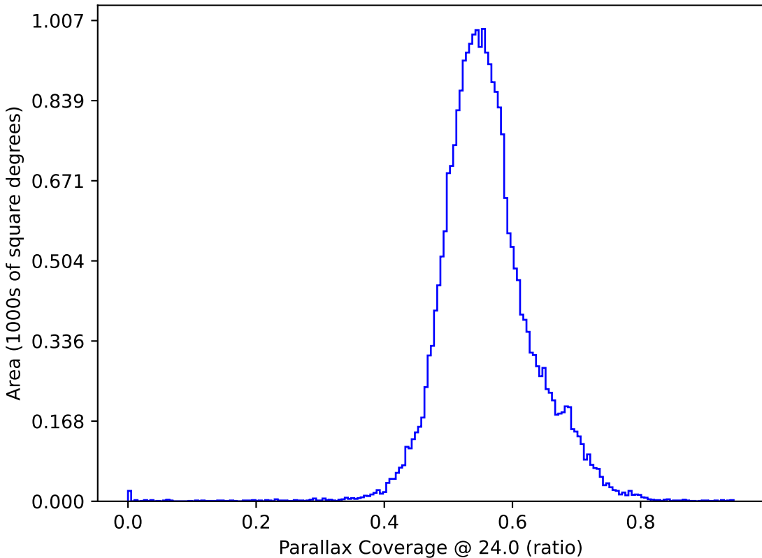
smc_lmc_v3.3_10yrs All sky: Parallax Coverage @ 24.0
