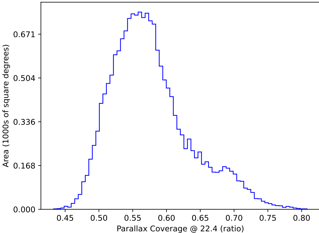
smc_lmc_v3.3_10yrs WFD: Parallax Coverage @ 22.4
