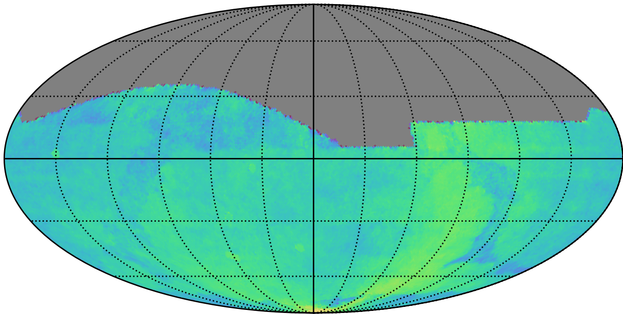
smc_lmc_v3.3_10yrs All sky: Parallax Coverage @ 22.4
