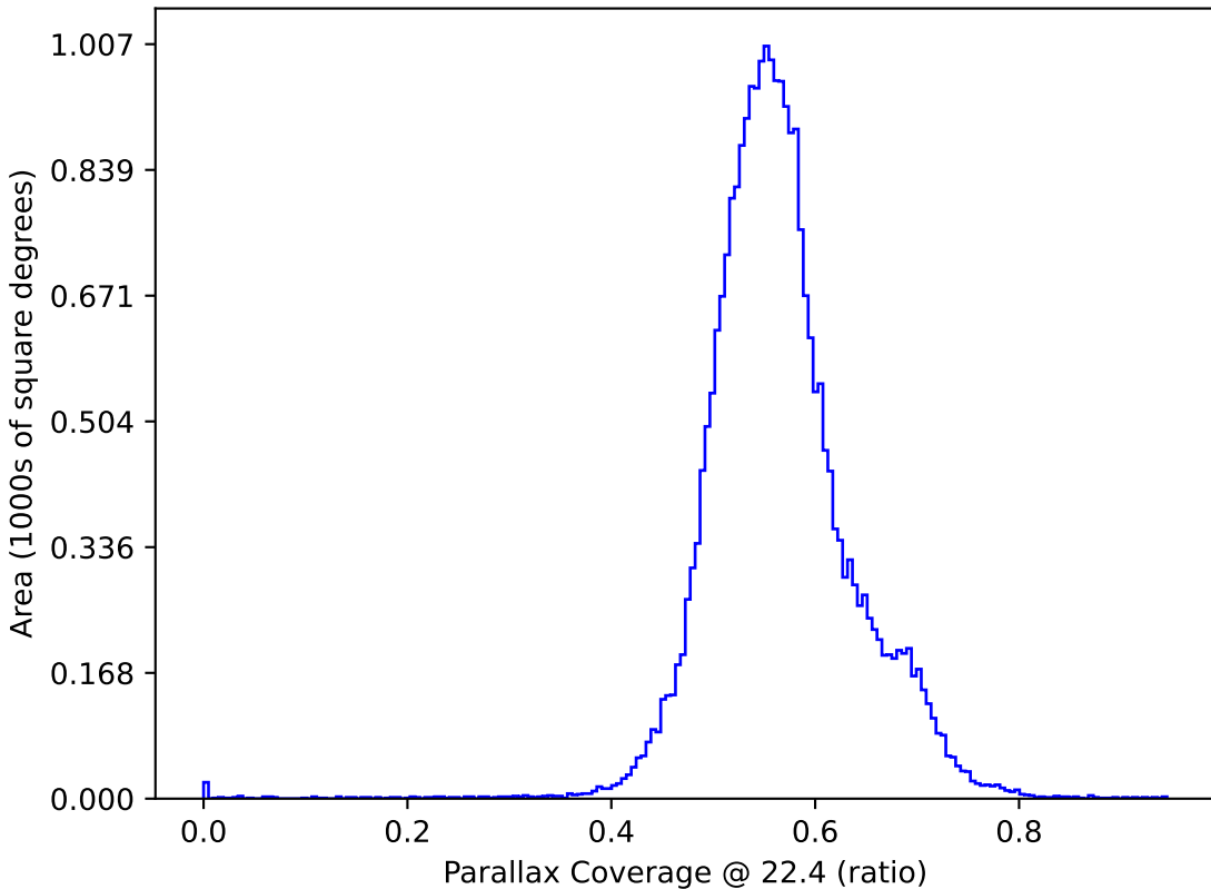
smc_lmc_v3.3_10yrs All sky: Parallax Coverage @ 22.4
