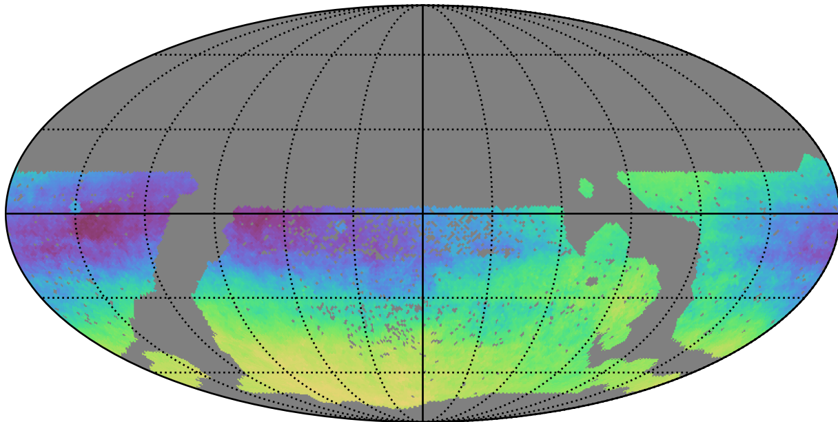
smc_lmc_v3.3_10yrs WFD: Parallax-DCR degeneracy @ 24.0
