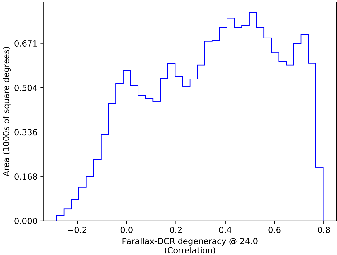
smc_lmc_v3.3_10yrs WFD: Parallax-DCR degeneracy @ 24.0
