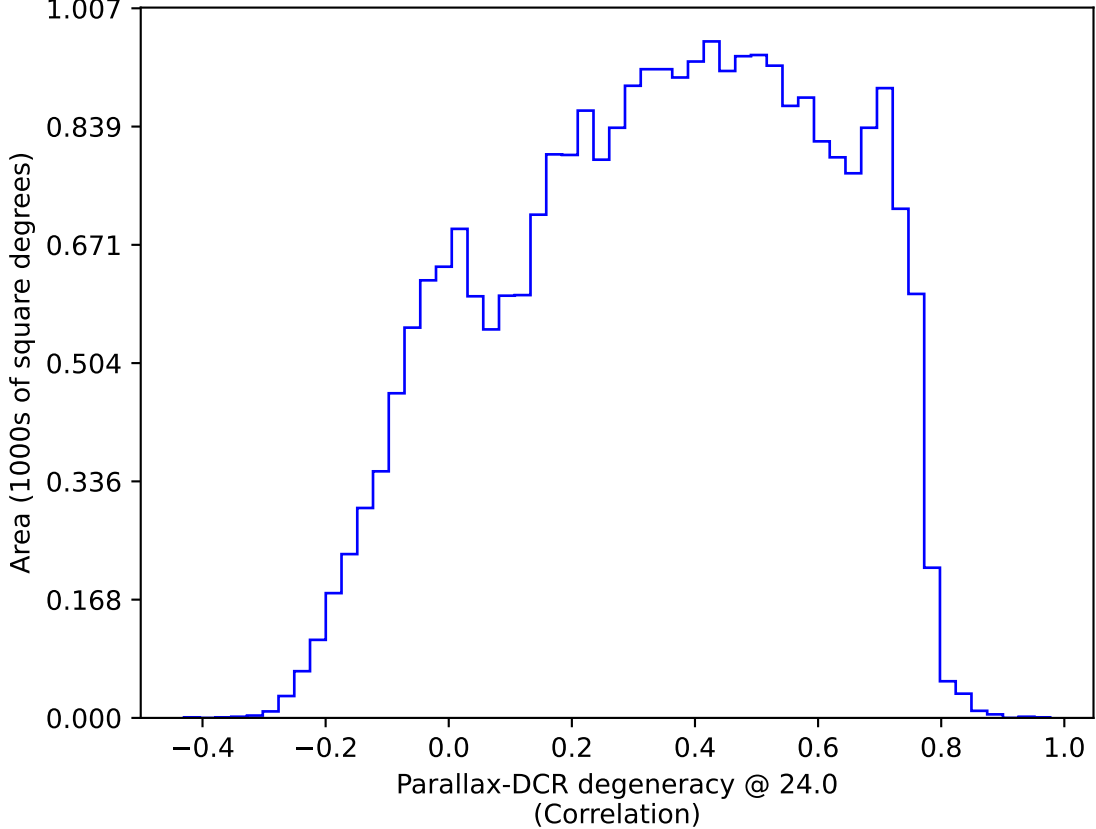
smc_lmc_v3.3_10yrs All sky: Parallax-DCR degeneracy @ 24.0
