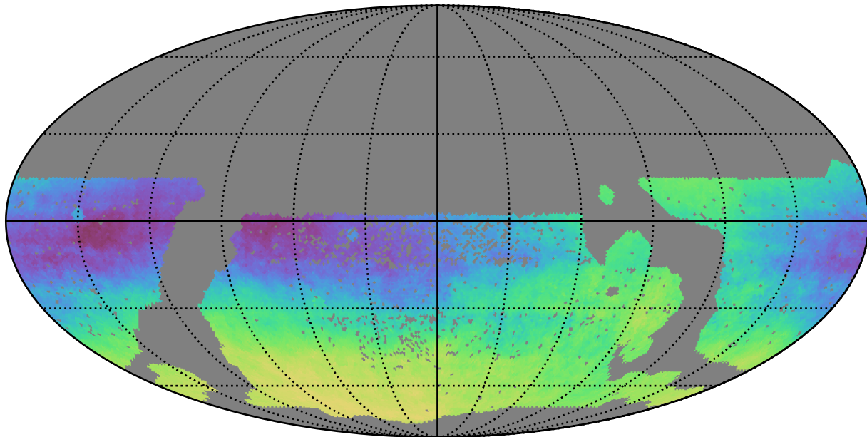
smc_lmc_v3.3_10yrs WFD: Parallax-DCR degeneracy @ 22.4
