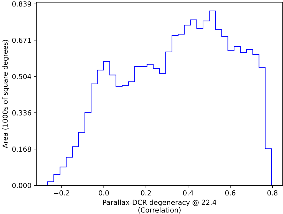
smc_lmc_v3.3_10yrs WFD: Parallax-DCR degeneracy @ 22.4
