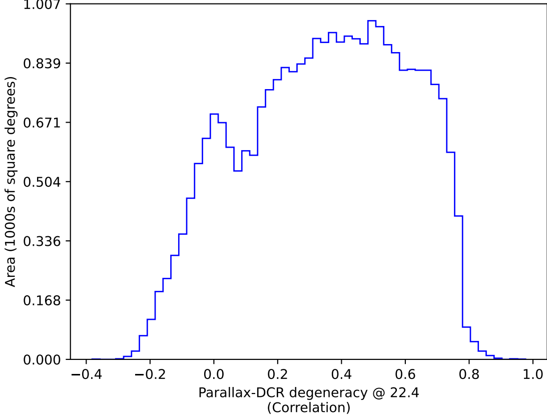
smc_lmc_v3.3_10yrs All sky: Parallax-DCR degeneracy @ 22.4
