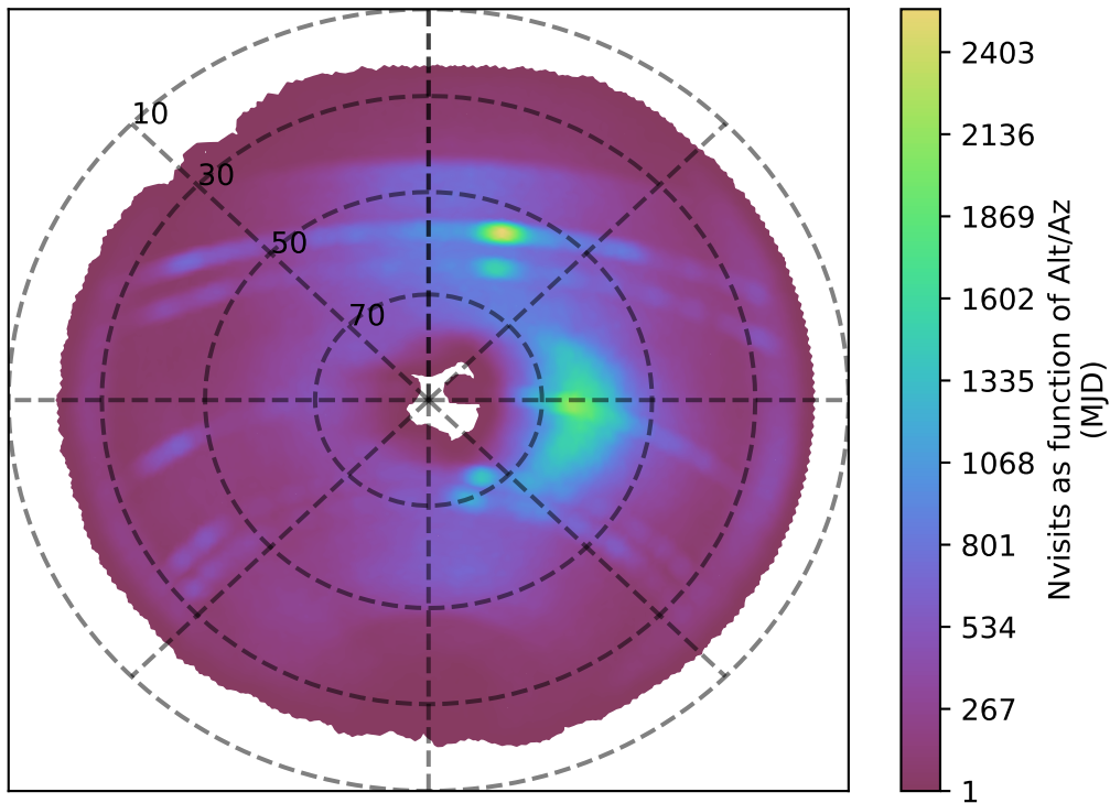
smc_lmc_v3.3_10yrs z band: Nvisits as function of Alt/Az
