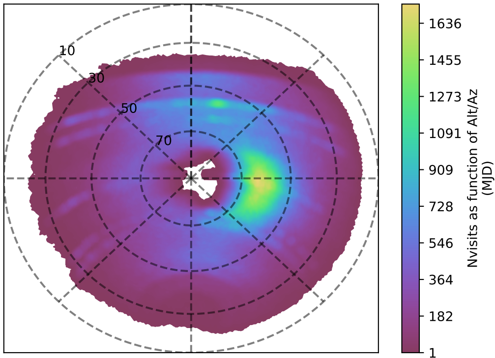
smc_lmc_v3.3_10yrs y band: Nvisits as function of Alt/Az
