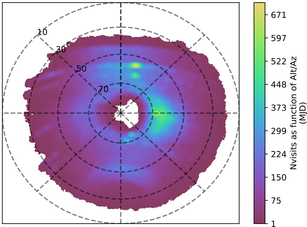
smc_lmc_v3.3_10yrs u band: Nvisits as function of Alt/Az
