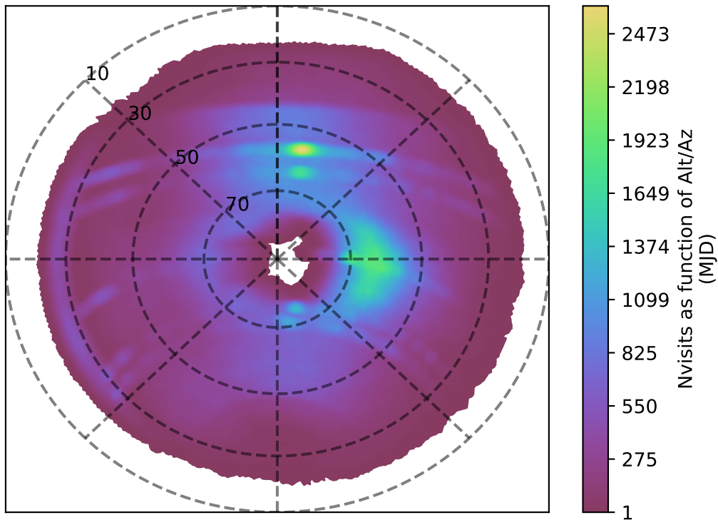
smc_lmc_v3.3_10yrs r band: Nvisits as function of Alt/Az
