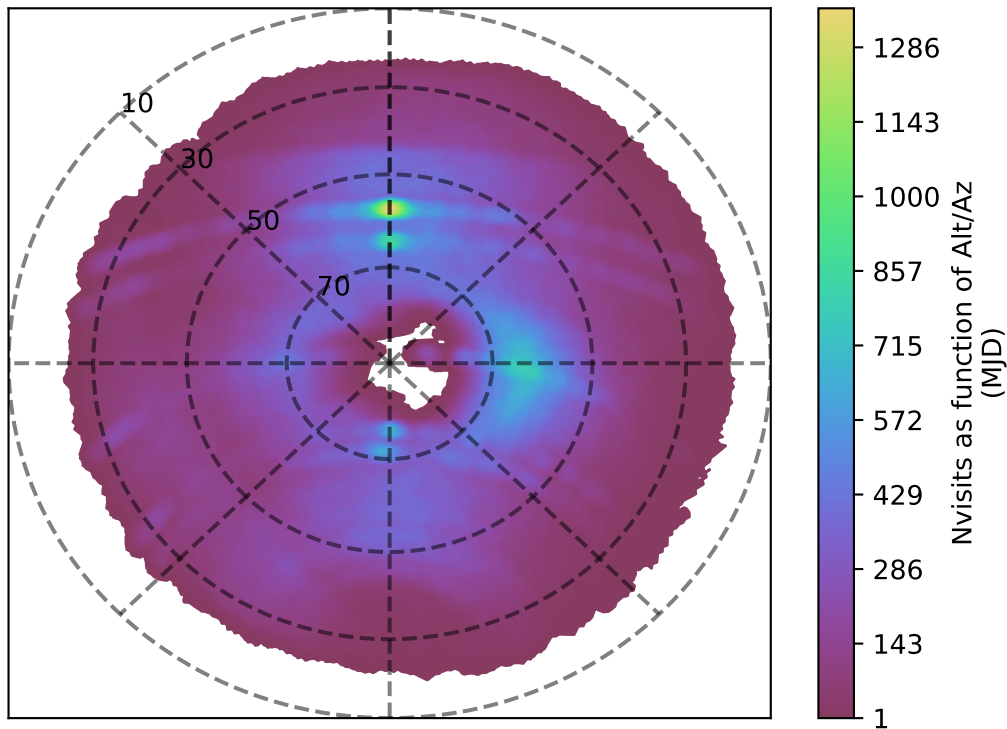
smc_lmc_v3.3_10yrs g band: Nvisits as function of Alt/Az
