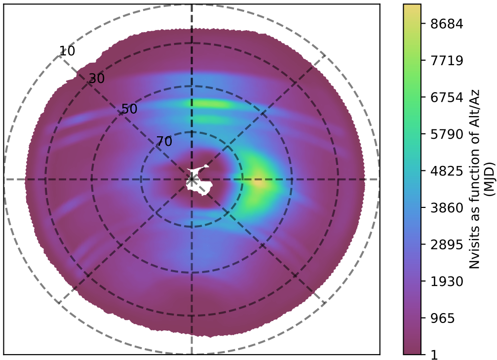
smc_lmc_v3.3_10yrs all bands: Nvisits as function of Alt/Az
