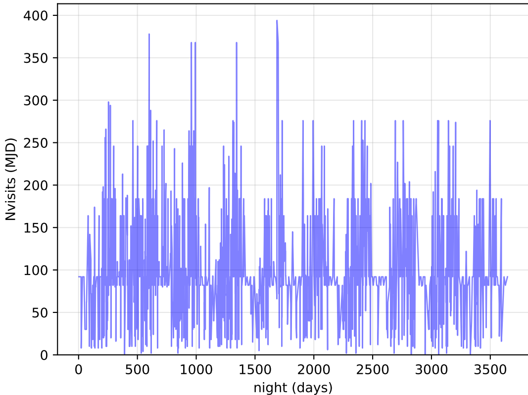
smc_lmc_v3.3_10yrs DDF: Nvisits
