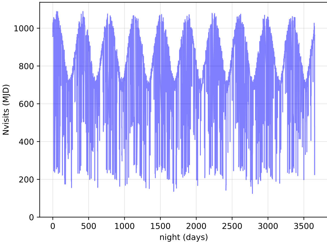
smc_lmc_v3.3_10yrs All visits: Nvisits
