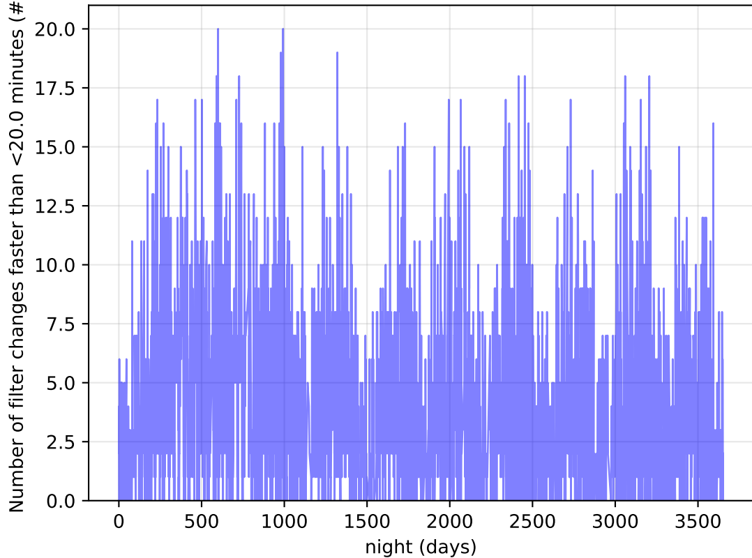
smc_lmc_v3.3_10yrs Per Night: Number of filter changes faster than <20.0 minutes
