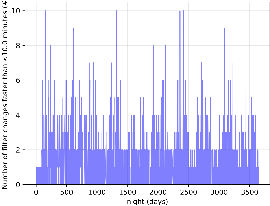
smc_lm_v3.3_10yrs Per Night: Number of filter changes faster than <10.0 minutes
