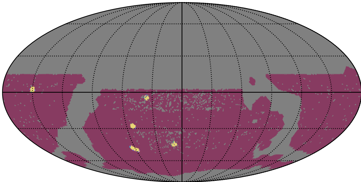
smc_lmc_v3.3_10yrs WFD: NumberOfQuickRevisits
