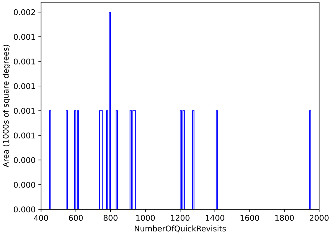
smc_lmc_v3.3_10yrs WFD: NumberOfQuickRevisits
