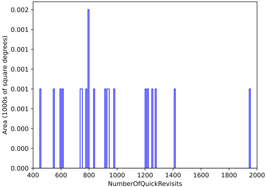
smc_lmc_v3.3_10yrs All sky: NumberOfQuickRevisits
