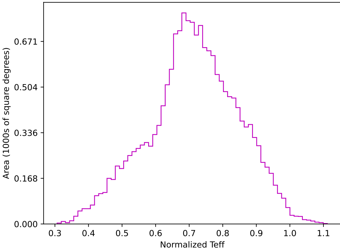
smc_lmc_v3.3_10yrs WFD z band: Normalized Teff
