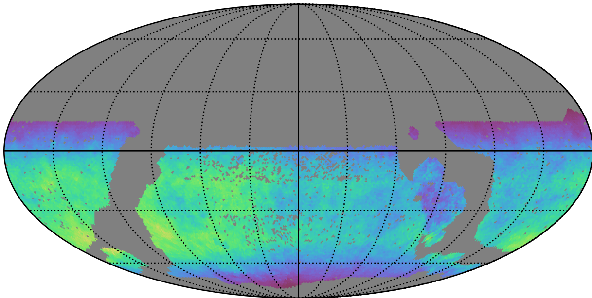
smc_lmc_v3.3_10yrs WFD y band: Normalized Teff
