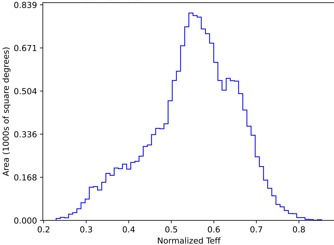
smc_lmc_v3.3_10yrs WFD y band: Normalized Teff
