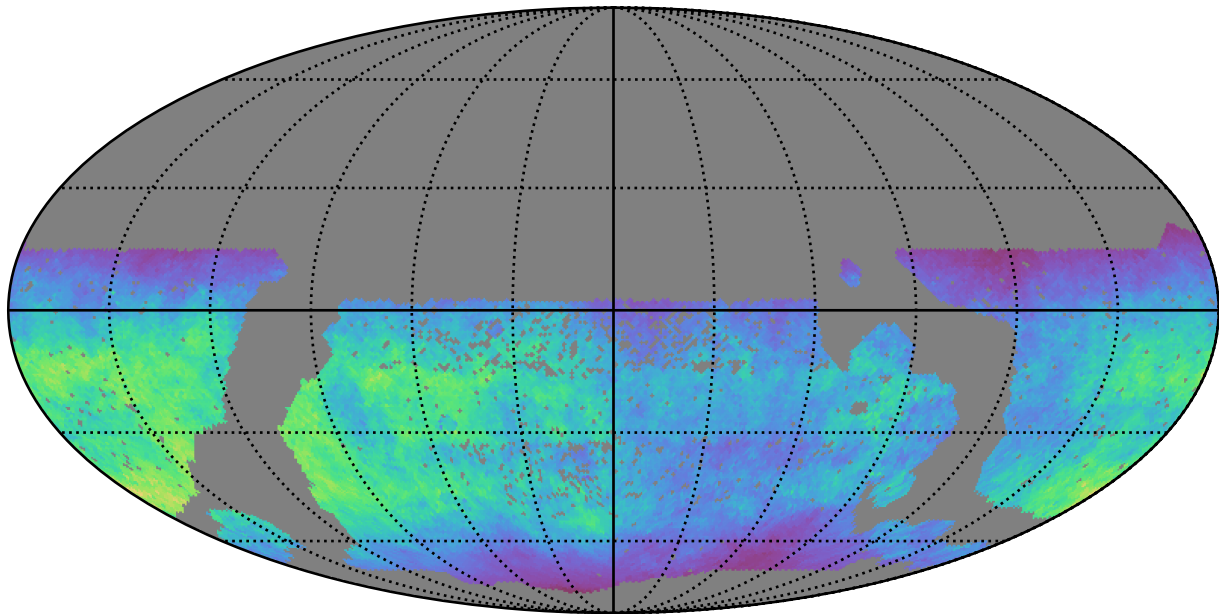
smc_lmc_v3.3_10yrs WFD u band: Normalized Teff
