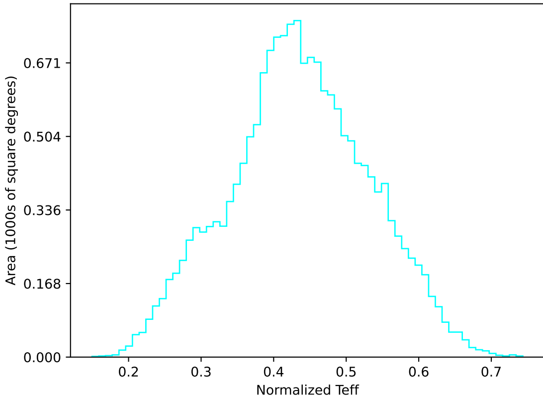
smc_lmc_v3.3_10yrs WFD u band: Normalized Teff
