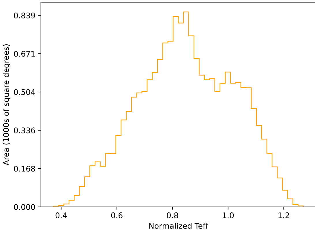
smc_lmc_v3.3_10yrs WFD r band: Normalized Teff
