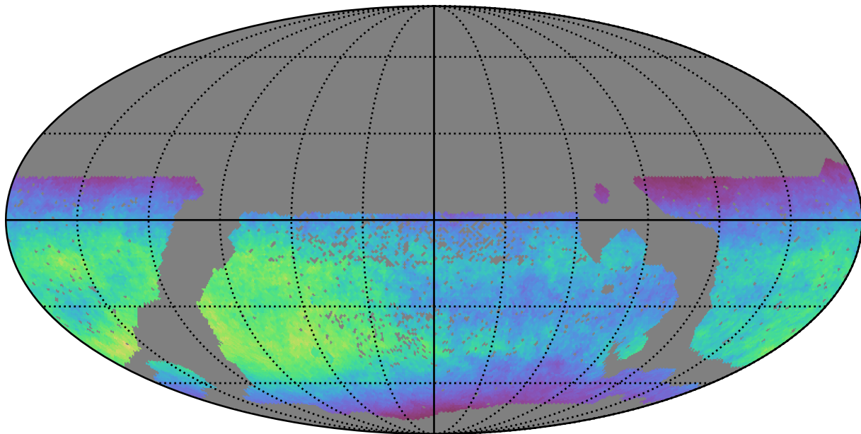
smc_lmc_v3.3_10yrs WFD i band: Normalized Teff
