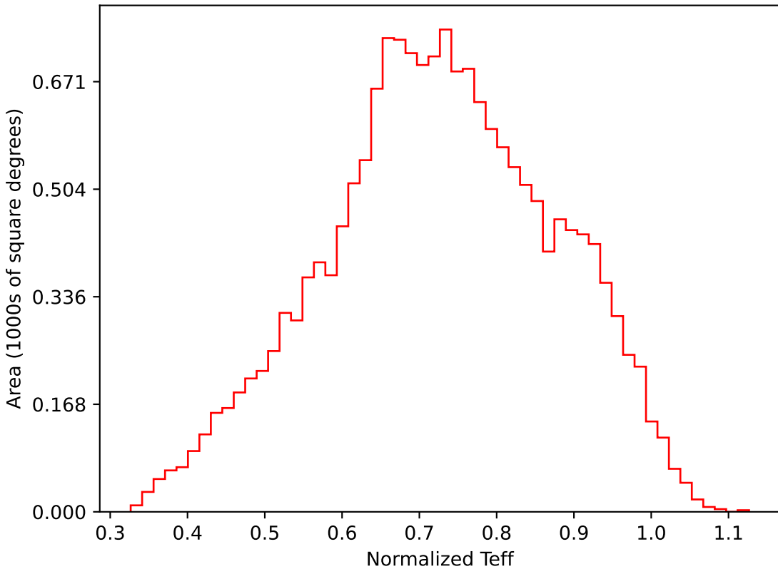
smc_lmc_v3.3_10yrs WFD i band: Normalized Teff
