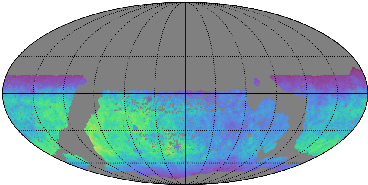
smc_lmc_v3.3_10yrs WFD g band: Normalized Teff
